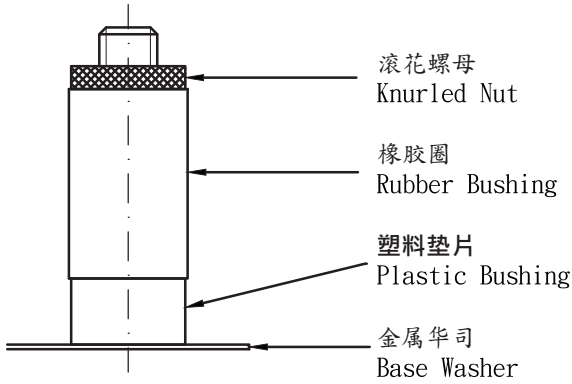
APP四件套 Rubber Expanding Adapters
