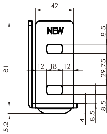
2孔规格 Two Holes Specification
