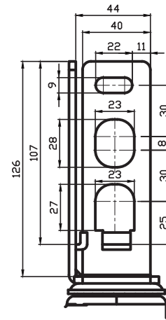
3孔规格 Three Holes Specification
